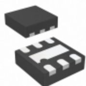
MIC5339-MGYMT-TR Microchip Technology IC REG LDO 2.8V/1.8V 0.3A 6TMLF
