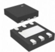
MIC5393-GMYMT-T5 Microchip Technology IC REG LDO 1.8V/2.8V 0.15A 6MLF
