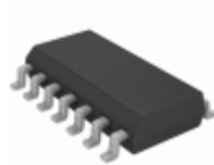
MCP4231T-503E/SL Microchip Technology IC DGTL POT 50K 2CH 14SOIC
