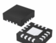
MCP4231T-502E/ML Microchip Technology IC POT DGTL DUAL 5K SPI 16QFN
