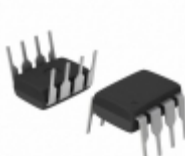
TC4424CPA Microchip Technology IC MOSFET DVR 3A DUAL HS 8-DIP
