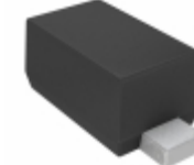
CDZVT2R12B Rohm Semiconductor DIODE ZENER 12V 100MW VMN2M
