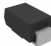
SMAJ17AHE3/5A Vishay Semiconductor Diodes Division TVS DIODE 17VWM 27.6VC SMA
