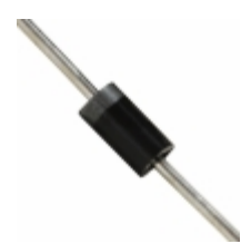
1N4761A BK Central Semiconductor Corp DIODE ZENER 75V 1W DO41
