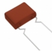
ECW-F2274RHA Panasonic Electronic Components CAP FILM 0.27UF 3% 250VDC RADIAL
