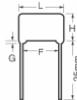
ECQ-P1H121JZ3 Panasonic Electronic Components CAP FILM 120PF 5% 50VDC RADIAL
