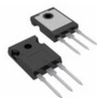
IRGP4790DPBF Infineon Technologies IGBT 650V TO-247
