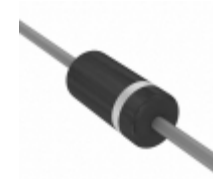
P6KE16CA-E3/73 Vishay Semiconductor Diodes Division TVS DIODE 13.6VWM 22.5VC DO204AC
