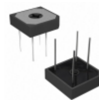
VS-GBPC2504W Vishay Semiconductor Diodes Division RECT BRIDGE 1-PH 400V 25A GBPCW
