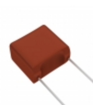
ECW-F2475HA Panasonic Electronic Components CAP FILM 4.7UF 3% 250VDC RADIAL
