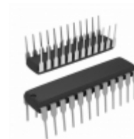
AT28BV16-30PI Microchip Technology IC EEPROM 16KBIT 300NS 24DIP
