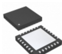
PIC18F27J53T-I/ML Microchip Technology IC MCU 8BIT 128KB FLASH 28QFN
