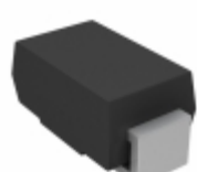
SML4744A-E3/5A Electro-Films (EFI) / Vishay DIODE ZENER 15V 1W DO214AC
