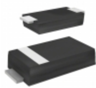
CZRA4732-G Comchip Technology DIODE ZENER 4.7V 1W DO214AC
