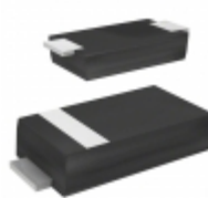
CZRA4733-G Comchip Technology DIODE ZENER 5.1V 1W DO214AC
