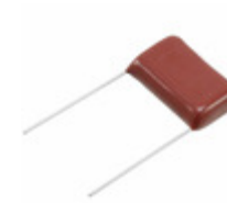
ECQ-E6474JFW Panasonic Electronic Components CAP FILM 0.47UF 5% 630VDC RADIAL
