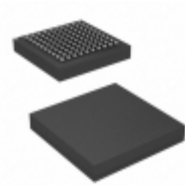
CY8C24094-24BVXIT Cypress Semiconductor Corp IC MCU 8BIT 16KB FLASH 100VFBGA
