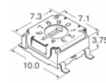
SH-7040TB Copal Electronics Inc. SW ROTARY DIP GRAY CODE 100MA 5V
