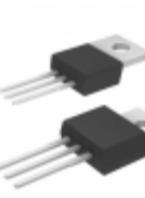
IXFP10N80P IXYS MOSFET N-CH 800V 10A TO-220
