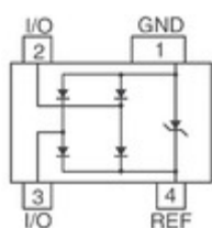
CD143A-SR05 Bourns Inc. TVS DIODE 5VWM 20VC SOT143
