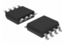
MC78L05ABDR2G ON Semiconductor IC REG LDO 5V 0.1A 8SOIC
