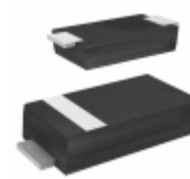
CZRA4732-G Comchip Technology DIODE ZENER 4.7V 1W DO214AC
