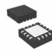
ISL6291-2CRZ Intersil IC CHARGER LI-ION 4.2V 5X5 16QFN
