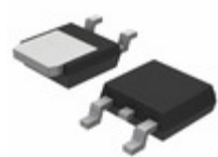
SURD8530T4G-VF01 ON Semiconductor DIODE GEN PURP 300V 5A DPAK
