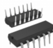
PIC16LC505-04/P Microchip Technology IC MCU 8BIT 1.5KB OTP 14DIP
