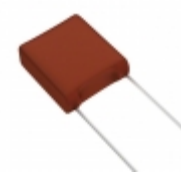
ECW-FA2J104J5 Panasonic Electronic Components CAP FILM 0.1UF 5% 630VDC RADIAL
