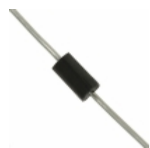
BYW100-200RL STMicroelectronics DIODE GEN PURP 200V 1.5A DO15
