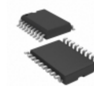
PIC16C620T-20/SO Microchip Technology IC MCU 8BIT 896B OTP 18SOIC
