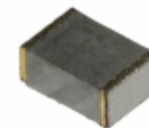
ECW-U2122V16 Panasonic Electronic Components CAP FILM 1200PF 5% 250VDC 1913
