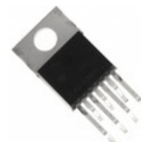
CS8151YTHA7G ON Semiconductor IC REG LDO 5V 0.1A TO220-7
