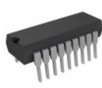
PIC16CE624-20E/P Microchip Technology IC MCU 8BIT 1.75KB OTP 18DIP
