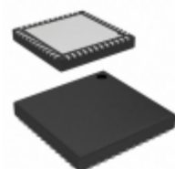
CY8C20636A-24LQXIT Cypress Semiconductor Corp IC CAPSENCE 1.8V 36 I/O 48QFN
