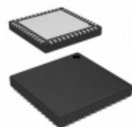
CY8C20646A-24LQXIT Cypress Semiconductor Corp IC CAPSENCE 1.8V 36 I/O 48-QFN
