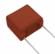
ECW-FA2J684J5 Panasonic Electronic Components CAP FILM 0.68UF 5% 630VDC RADIAL
