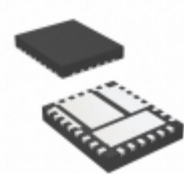
MIC24055YJL-TR Microchip Technology IC REG BUCK ADJ 12A SYNC 28QFN
