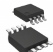
MCP4541T-103E/MSVAO Micrel / Microchip Technology IC POT DGTL 10K SGL 8-MSOP
