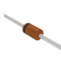
MTZJ9V1SA R0G TSC (Taiwan Semiconductor) DIODE ZENER 8.51V 500MW DO34
