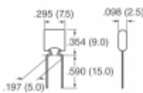
B37984M5334M051 EPCOS (TDK) CAP CER 0.33UF 50V X7R RADIAL
