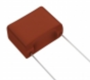
ECW-F2W475JA Panasonic Electronic Components CAP FILM 4.7UF 5% 450VDC RADIAL
