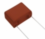
ECW-F2W475JA Panasonic Electronic Components CAP FILM 4.7UF 5% 450VDC RADIAL
