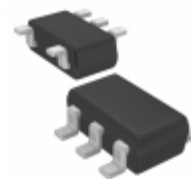
XC6123D328MR-G Torex Semiconductor Ltd IC WATCHDOG TIMER SOT-25
