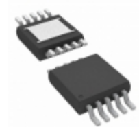
LTC1403AIMSE-1#TRPBF Linear Technology IC ADC 14BIT 2.8MSPS DIFF 10MSOP
