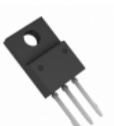
BA178M05CP-E2 Rohm Semiconductor IC REG LDO 5V 0.5A TO220CP-3
