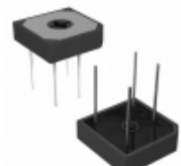
VS-GBPC3502W Electro-Films (EFI) / Vishay RECT BRIDGE GPP 35A 200V GBPCW
