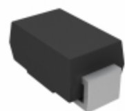
BZG03C220-HM3-18 Electro-Films (EFI) / Vishay DIODE ZENER 220V 1.25W DO214AC
