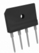
GBJ2506-G-04 Comchip Technology RECTIFIER BRIDGE 25A 600V GBJ
