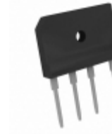
GBJ2506-06-G Comchip Technology RECTIFIER BRIDGE 25A 600V GBJ
