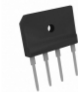
GBJ2506-G-05 Comchip Technology RECTIFIER BRIDGE 25A 600V GBJ
