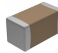
CDR32BP4R7BCWSAT Electro-Films (EFI) / Vishay CAP CER 4.7PF 100V BP 1206
