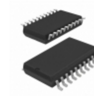
ADUM4152BRIZ-RL Analog Devices Inc. DGTL ISOLATOR 5KV 7CH SPI 20SOIC
