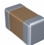
C0603C180J3HACAUTO KEMET CAP CER 0603 18PF 25V ULTRA STAB
