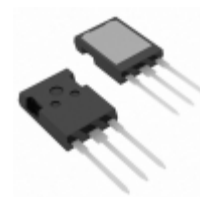
IXFX260N17T IXYS MOSFET N-CH 170V 260A PLUS247
